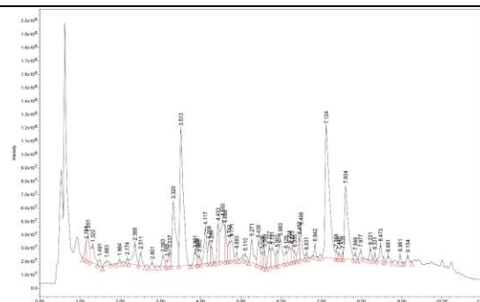
Figure 6. MS-TIC chromatogram of ArmF
